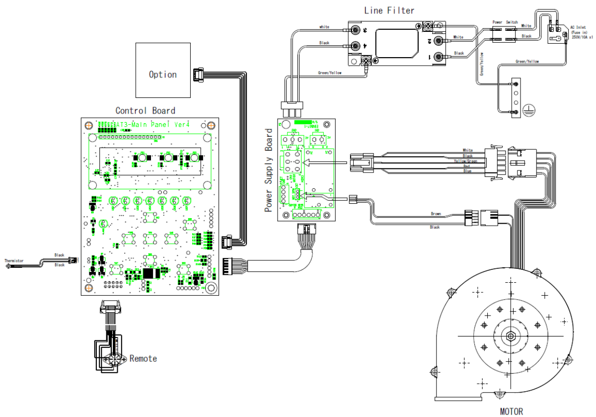
CBA-500AT3-HI(-T/-CE)
