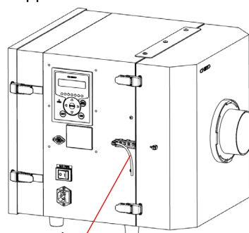
Out pressure sensing tube
